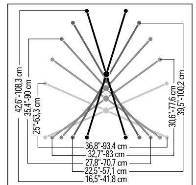
BS/619 Height & width positions
